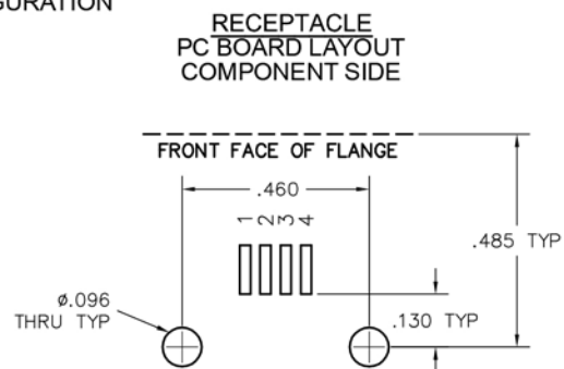
FOOTPRINT/PAD CONFIGURATION
