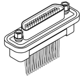
MM-2H2-031-261-26WA (RECEPTACLE)
