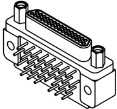
MK-2T2-031-335-220S (PLUG)
